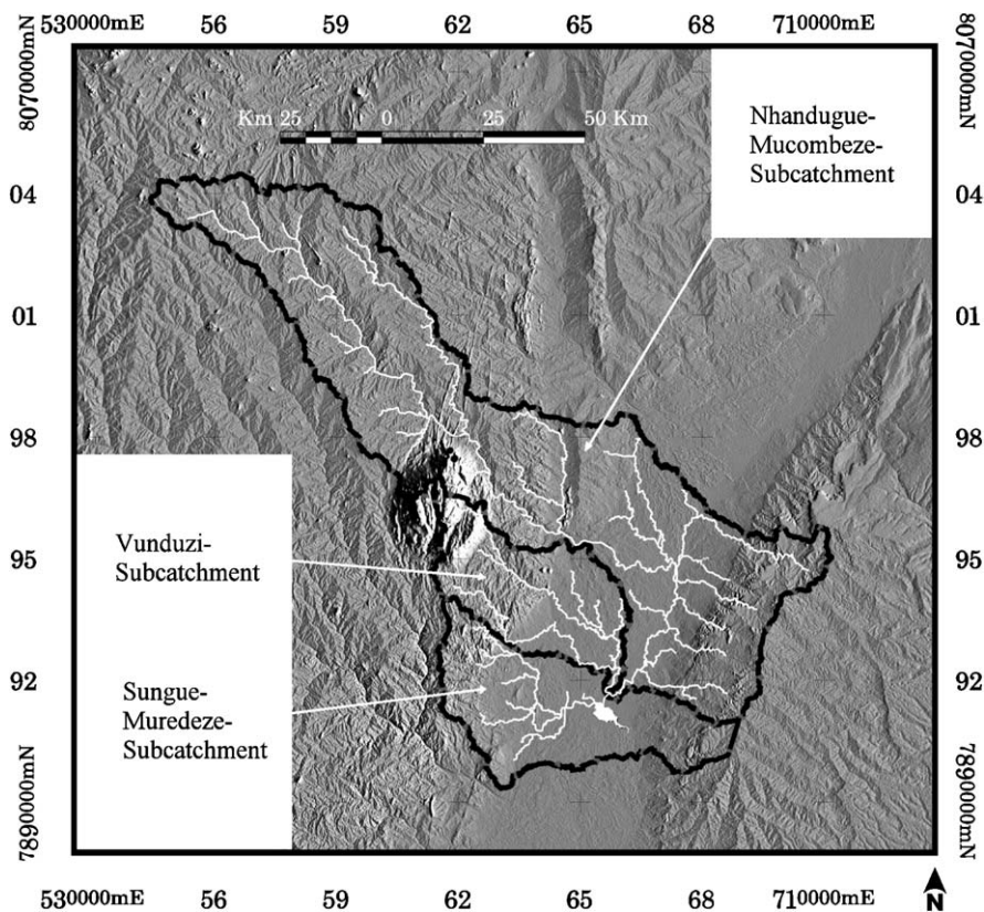
Fig. 2. Catchment area of the Lake Urema with sub-catchments and drainage system as derived from SRTM-DTM, sun elevation angle 30^\circ , sun azimuth angle 90^\circ .
