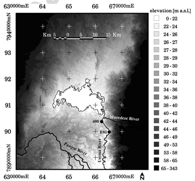
Fig. 8. Detail of the Urema basin from SRTM-DTM, showing flooded areas (in white) in May 1997.
