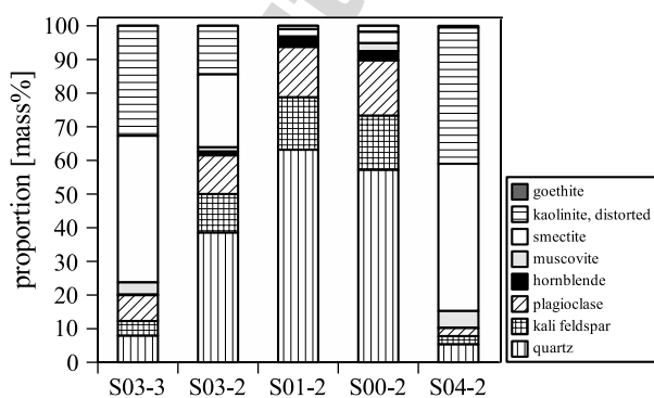
Fig. 5. Mineral composition of sampled sediment cores.
